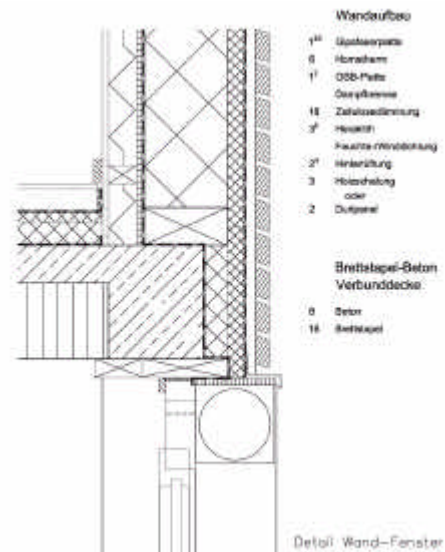
Abb. 13 Block 9 Detail Wand- Fenster
